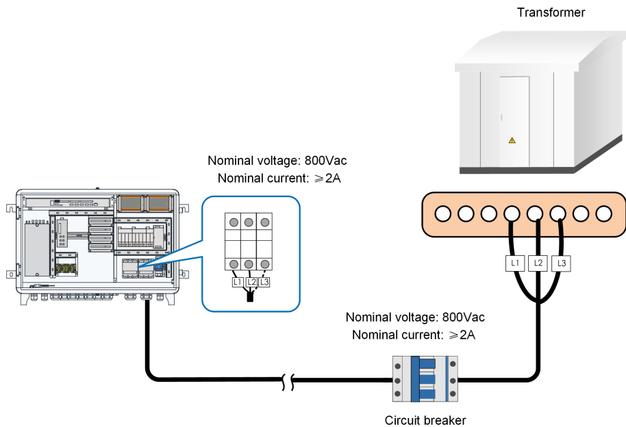
figure 4-11 Three-phase three-wire system
