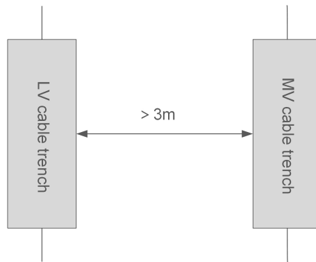
figure 4-6 Horizontal spacing between PLC cables (in parallel)
