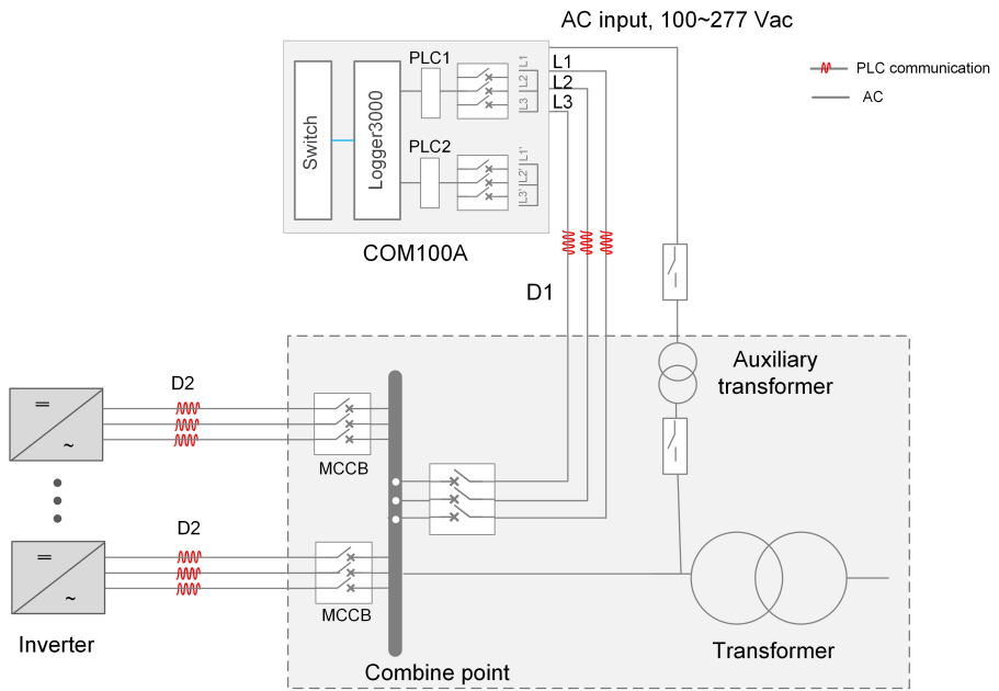
figure 4-1 PLC wiring diagram for a double-winding transformer
