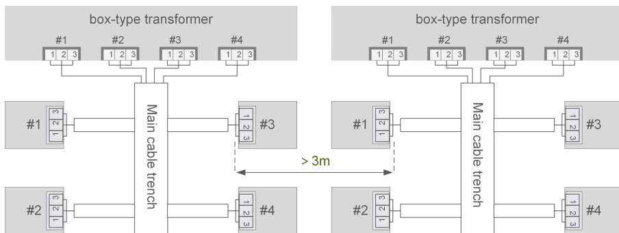
figure 4-8 Diagram of PLC wiring under different box-type transformers
