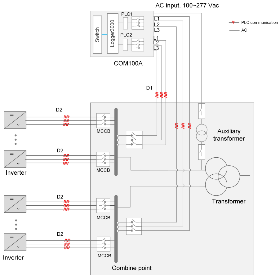
figure 4-2 PLC wiring diagram for a double-split transformer
