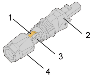
figure 4-1 SUNCLIX Connector Components
