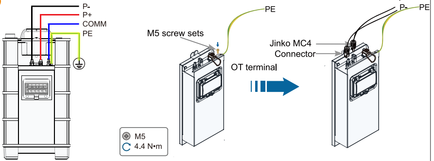
Connection Diagram
