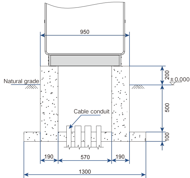
Figure 4-2 Foundation Dimensions (mm)
