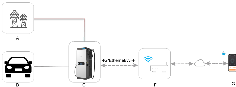
Figure 3-4 Remote Charging
