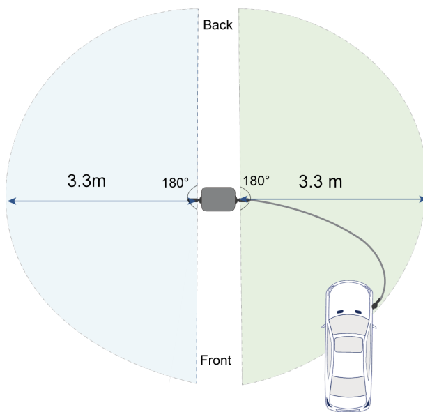
Figure 3-5 Actual working radius of the 5-meter cable
