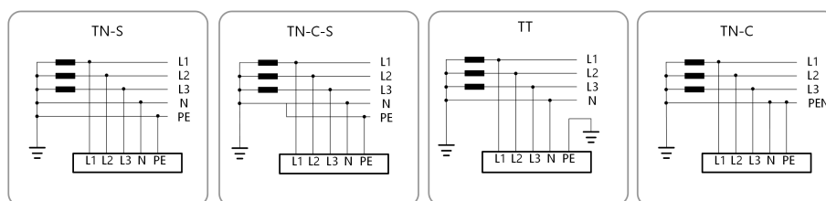
Figure 3-1 Earthing Systems
