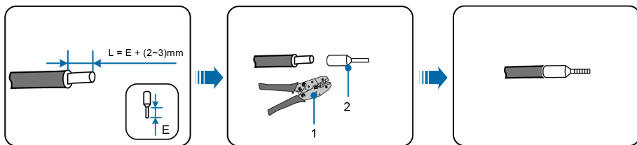
(1) Crimp tool
