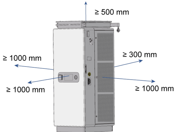
Figure 4-1 Space Requirements for Installation
