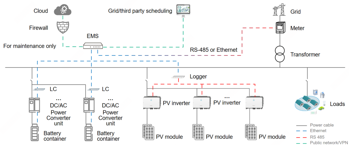
Fig. 4 Security Architecture for Commercial Scenarios
