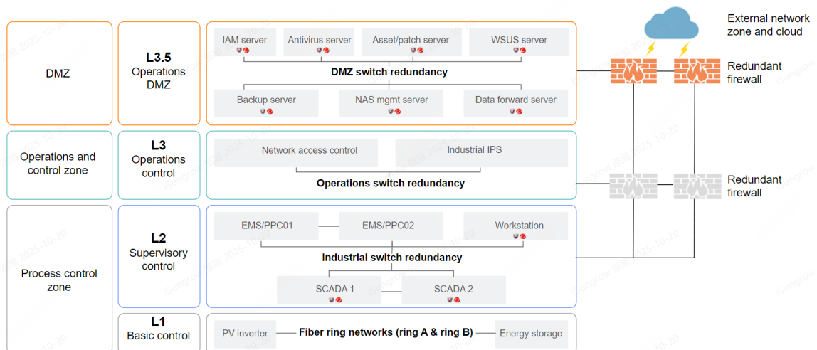
Fig. 5 Cybersecurity Architecture for Utility Systems
