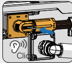
2-3 Connect the battery cable connector
