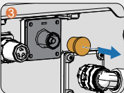
3-1 Remove the plug
