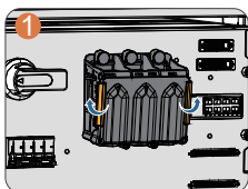
1 Release the snap-fits on the junction box
