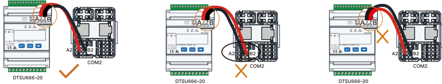
Cables connected in reverse at A2 and B2 on the inverter Cables connected in reverse at A and B on the meter
