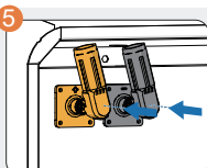
5 Attach the DC-side cable connectors of the DC/AC power converter unit
