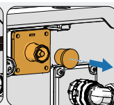
2-3 Remove the plug
