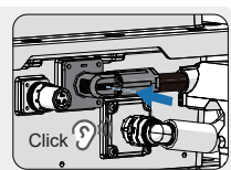
3-3 Attach the battery cable connector
