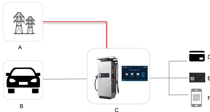
Figure 2-2 Near-end Charging
