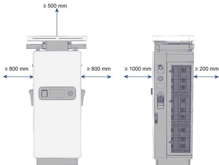
Figure 3-1 Space Requirements for Installation
