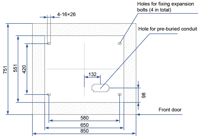
Figure 3-3 Location of Expansion Bolt Holes
