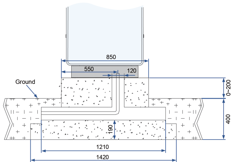
Figure 3-2 Foundation Dimensions (mm)
