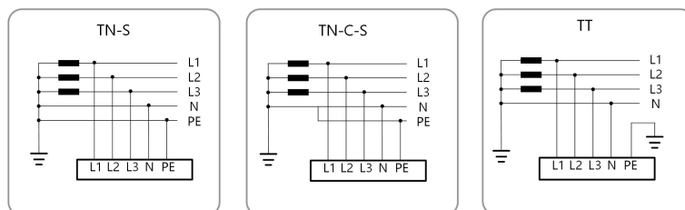
Figure 3-6 Earthing Systems
